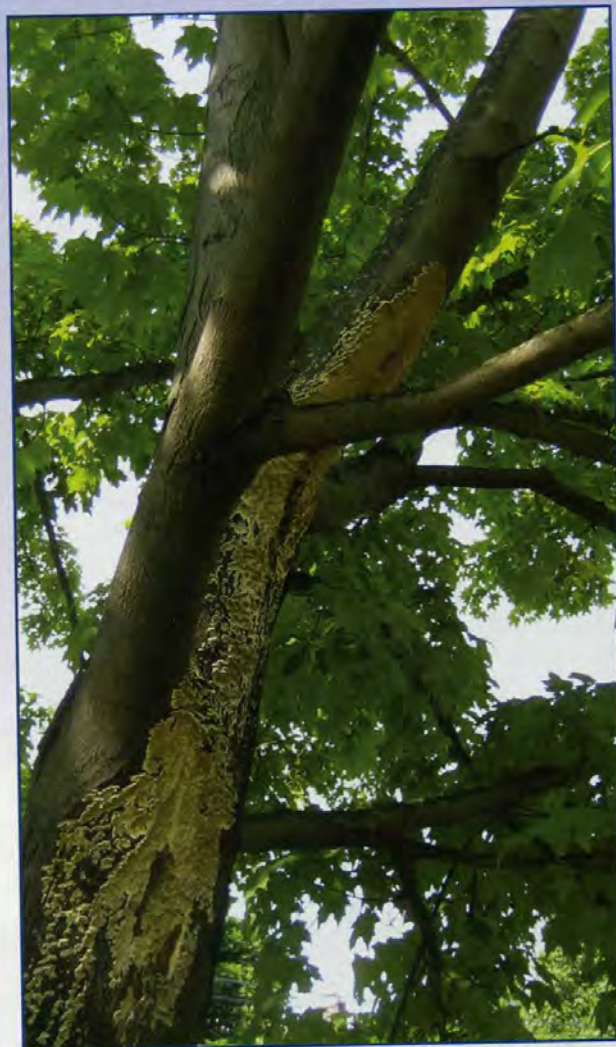
Figure 6. Sap rot caused by Irpex lacteus . The number of fungal species that cause sap rot is much greater than those that cause heart rot of living trees. Sap rot fungi have a wide variety of fruiting bodies but most produce a large number of small structures on wood.
